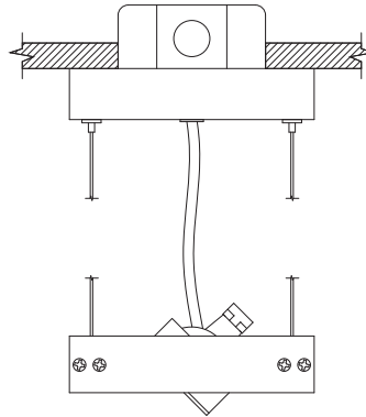
CABLE MOUNTING
